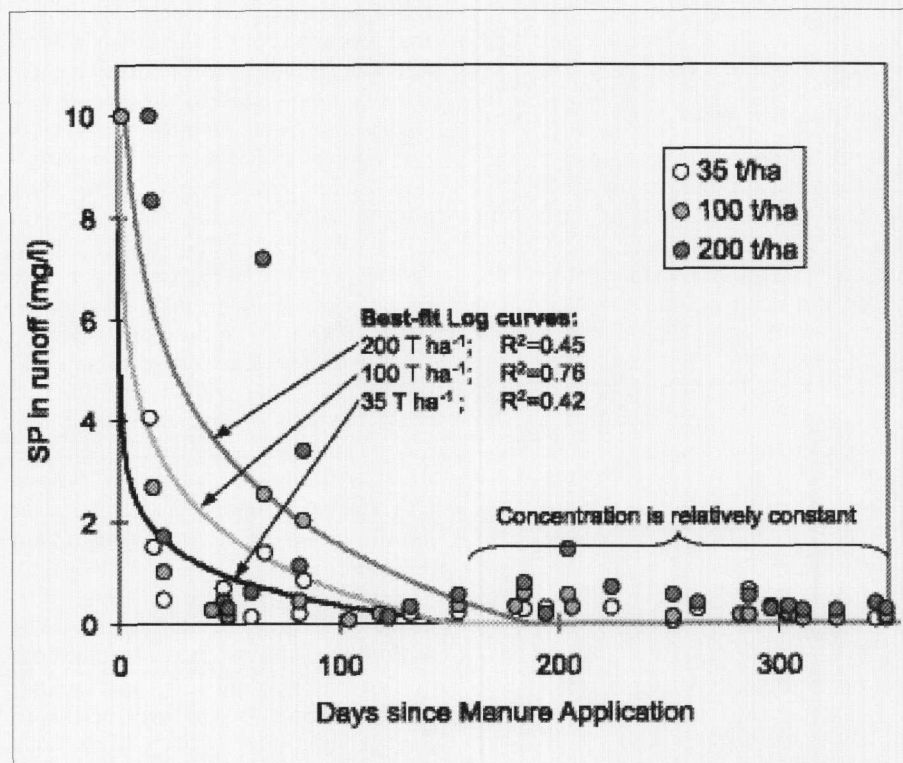
Figure 2. Dissolved phosphorus concentration in runoff vs. days since application for three application densities. Symbols are data: red=200 T ha -1 (220 Ton ac -1 ), blue = 100 T ha -1 (110 Ton ac -1 ), open = 35 T ha -1 (39 Ton ac -1 ). Lines are best-fit logarithmic curves.
