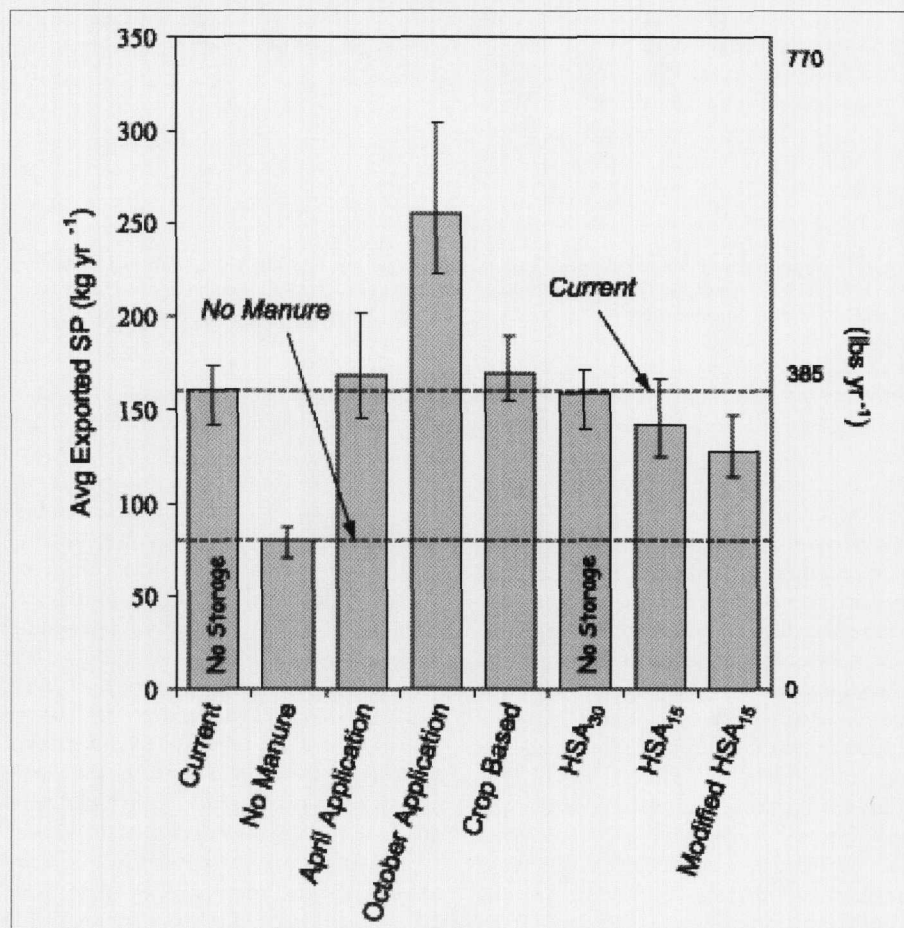
Figure 6. Predicted yearly averaged dissolved phosphorus exported from the farm during 1991 through 1995 (+/- 1 standard deviation error bars).
