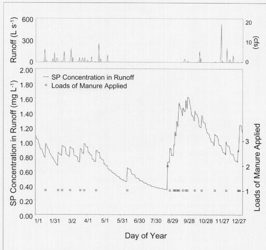
Figure 4. Example of predicted SP concentration in surface runoff from a field in the Catskills (1991) under the Current strategy. Note: 1 load of manure is 3 T (3.3 Ton).
