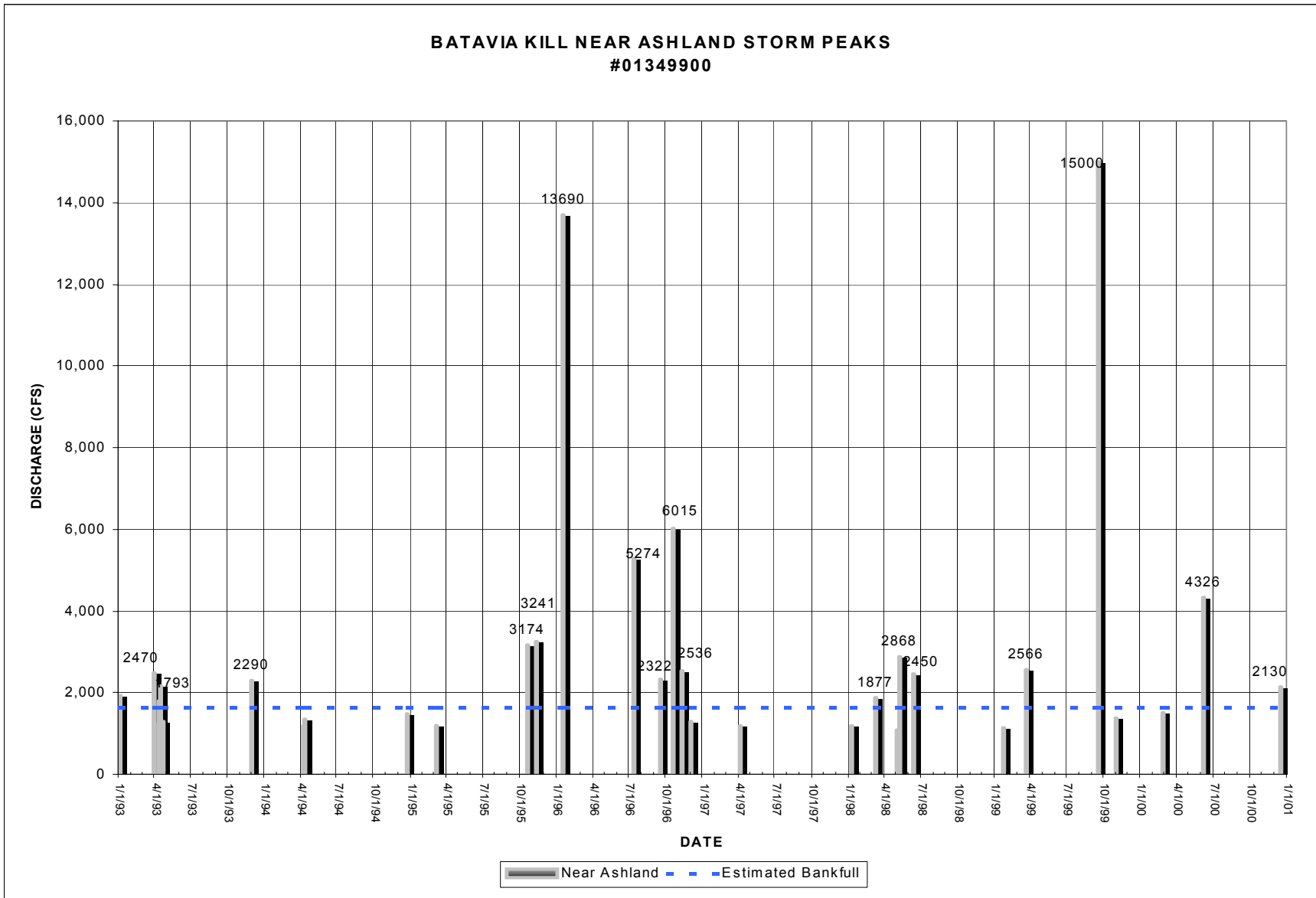
Figure V-20: Batavia Kill storm events over 1000cfs at Ashland, 1993-2001.
