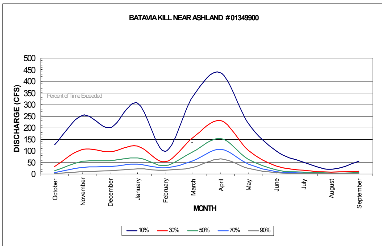
Figure V-17: Monthly probability curve for Near Ashland gage.
