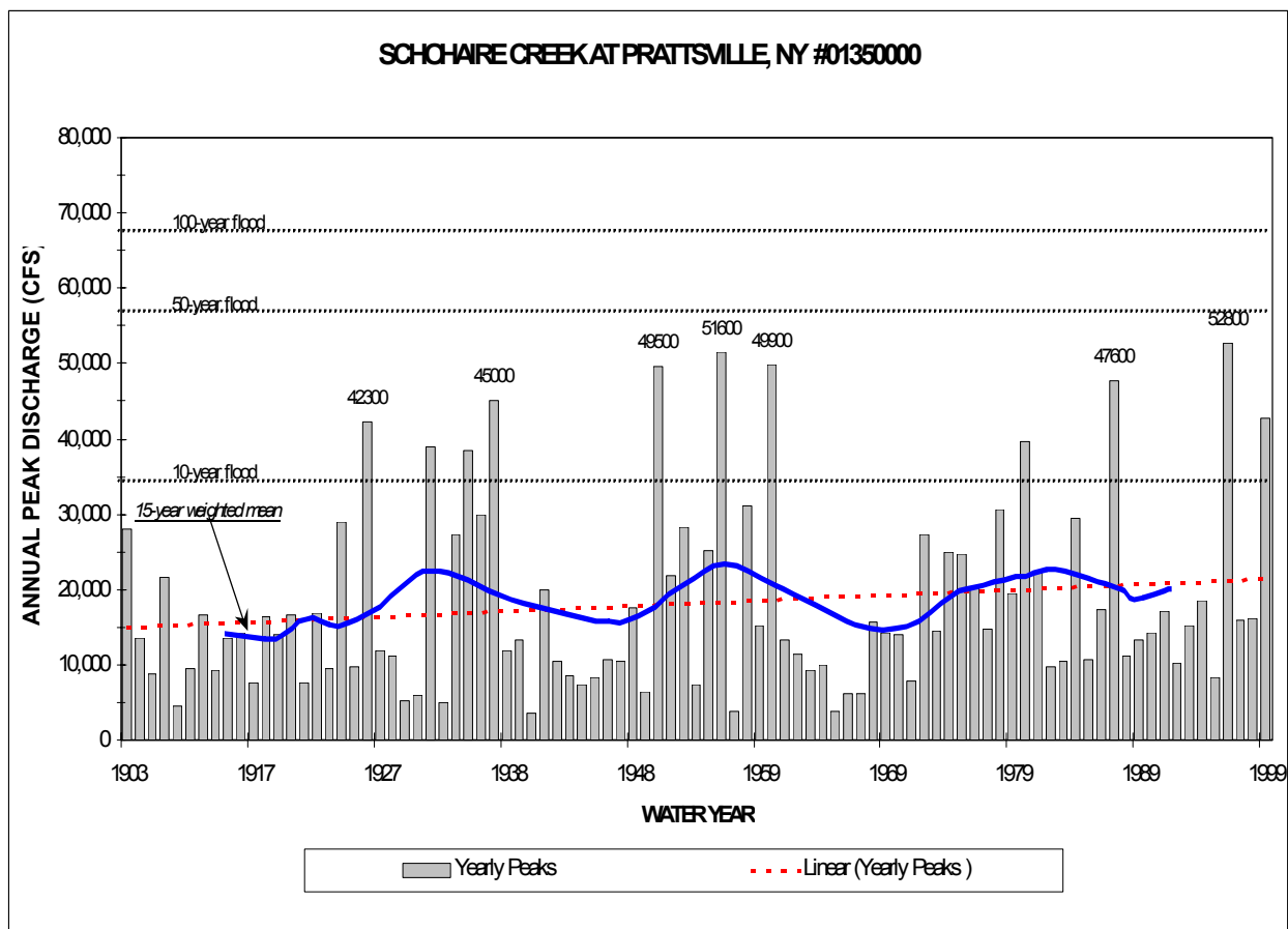
Figure V-15: Schoharie Creek historic yearly peak discharges.
