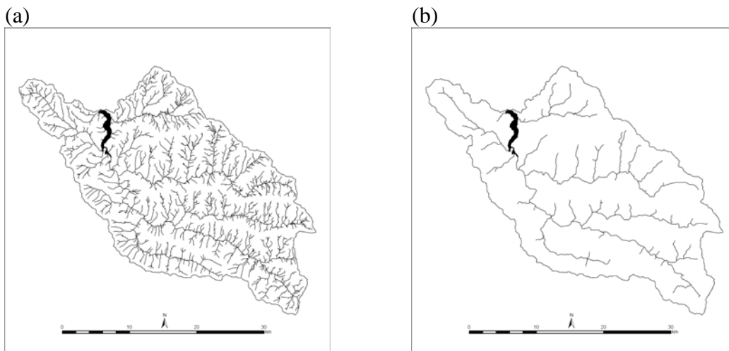
Figure 3.5. Schoharie watershed stream network: (a) all streams and (b) 3 rd order and above streams.
