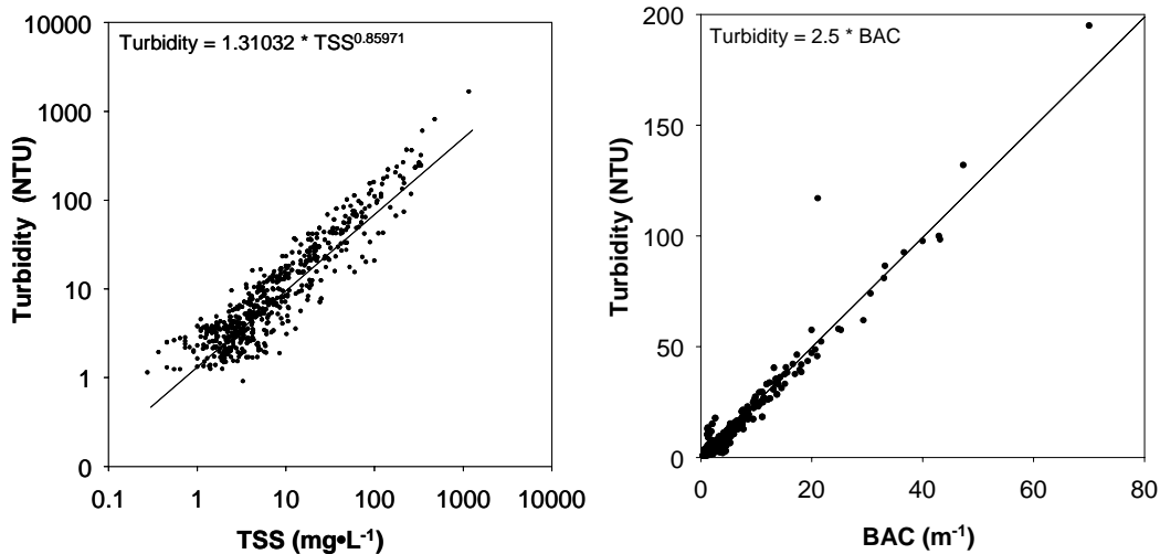
Figure 3.8. Relationships used to relate suspended sediment to turbidity (R. Gelda, personal communication, 2007) and beam attenuation coefficient (Effler et al., 2006).
