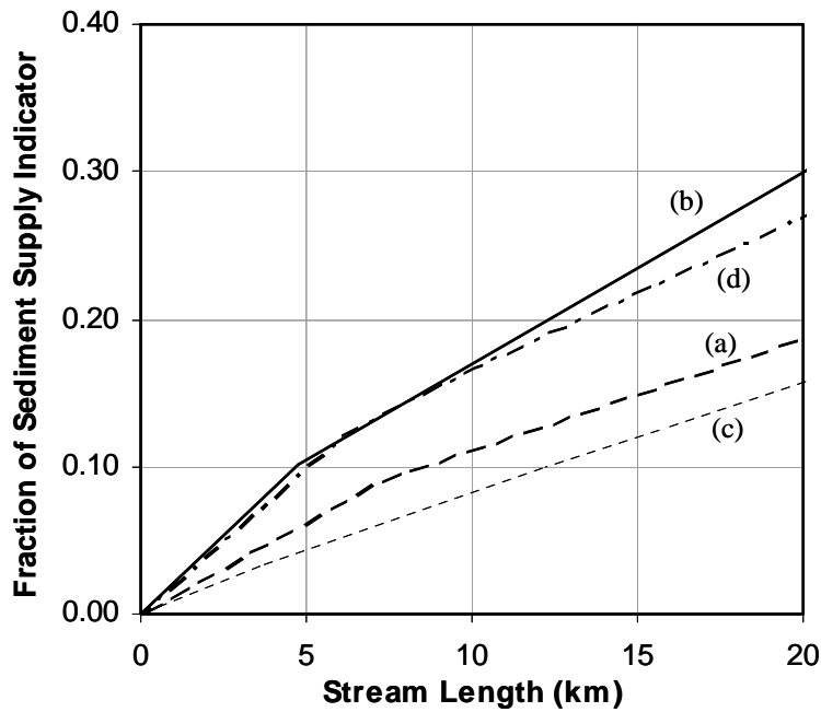
Figure 3.6. Cumulative distribution of indicators of sediment supply based on stream length: (a) wetted perimeter including all streams; (b) wetted perimeter only including 3 rd order and above streams; (c) percent of reach with active bank erosion and (d) percent of clay exposure
