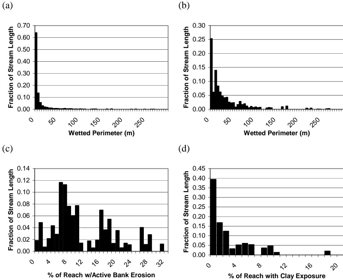
Figure 3.4. Histograms of indicators of sediment supply: (a) wetted perimeter including all streams; (b) wetted perimeter only including 3 rd order and above streams; (c) percent of reach with active bank erosion and (d) percent of clay exposures.
