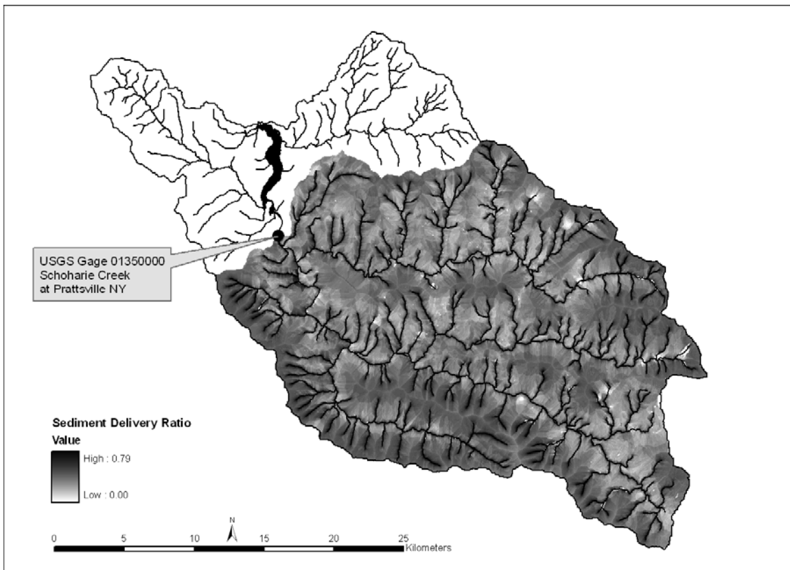
Figure 3.3. Map of sediment delivery ratio as calculated using SEDMOD (Fraser, 1999) for Schoharie Creek at Prattsville watershed.
