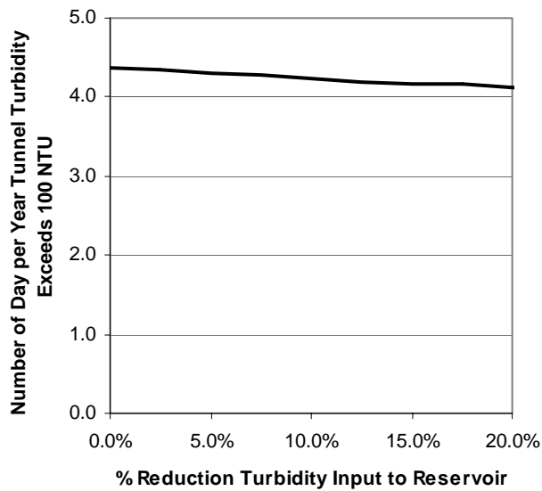
Figure 3.11. Sensitivity of the number of days that Shandaken Tunnel turbidity 100 NTU versus the percent reduction in turbidity input from Schoharie watershed.
