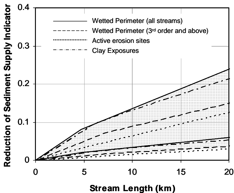
Figure 3.6. Cumulative distribution of indicators of sediment supply based on stream length: (a) wetted perimeter including all streams; (b) wetted perimeter only including 3 rd order and above streams; (c) percent of reach with active bank erosion and (d) percent of clay exposure
