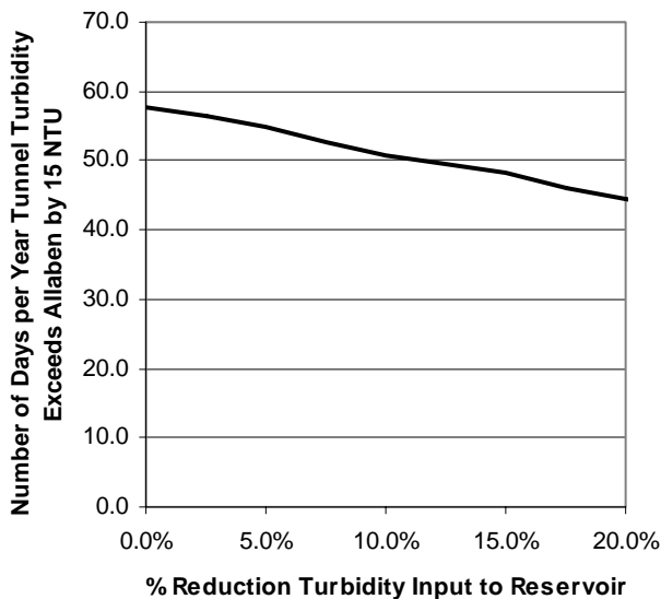
Figure 3.10. Sensitivity of the number of days that Shandaken Tunnel turbidity exceeds Esopus Creek at Allaben turbidity by at least 15 NTU versus the percent reduction in turbidity input from Schoharie watershed.
